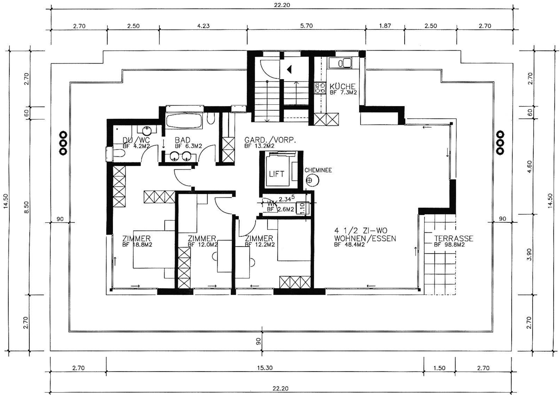
ATTIKAGESCHOSS 1:100
